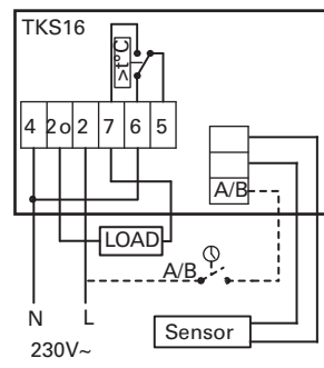
2-polig brytning / 2-pole switching
