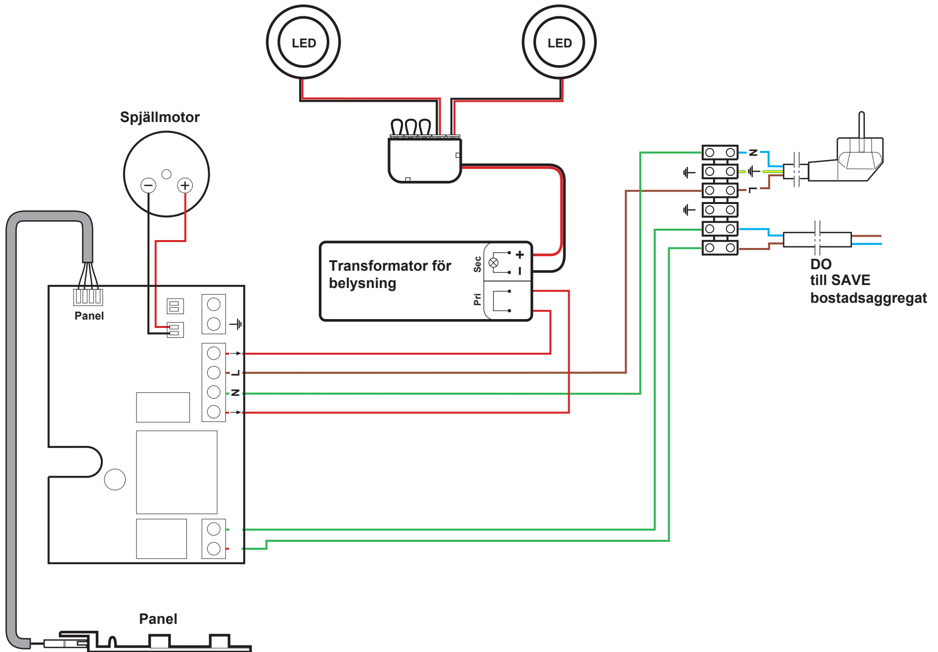
Wiring diagram 392-10
