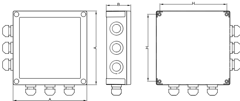
Fig. 4 Dimensions control board
