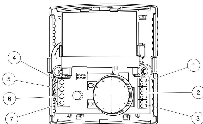
Fig. 6 Internal connections Room unit
