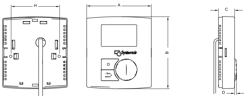
Fig. 3 Dimensions room unit
