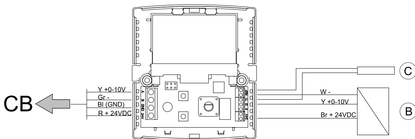
Fig. 8 Example of connection to external components on the room unit
