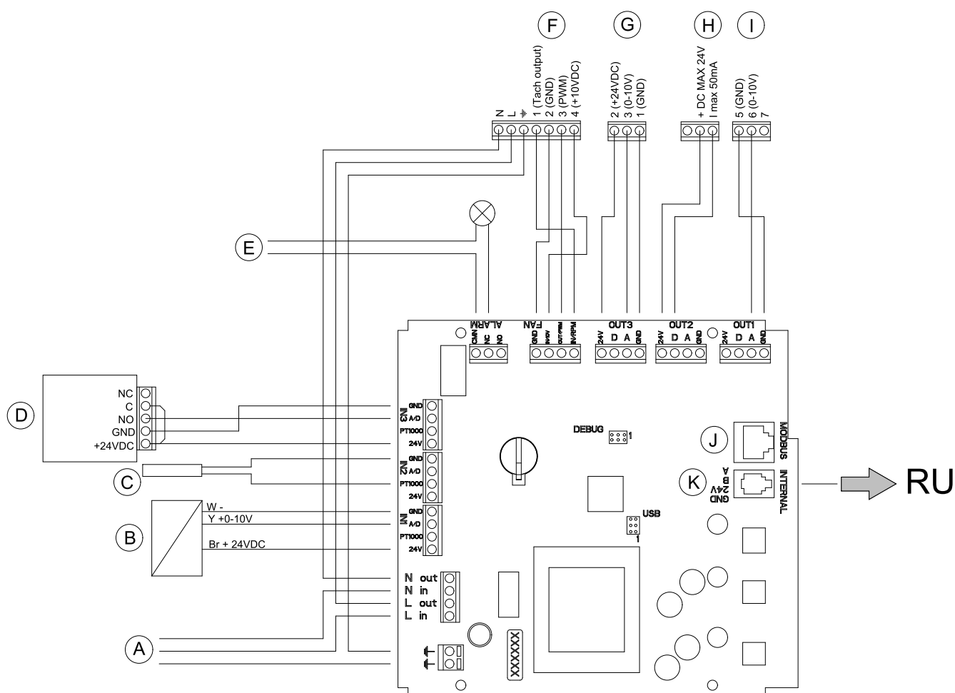
Fig. 7 Example of connection to external components on the control board
