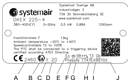
Fig. 3 Name plate
