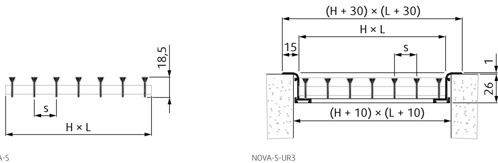
Fig. 8: Basic NOVA-S dimensions and grille types
