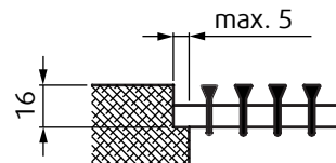
Fig. 7: The NOVA-S grille mounting directly into a window sill opening
