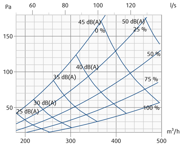
VVKR-B-S-400-16-B-SW + PB-VVK-S-400-200-S-H-D1
