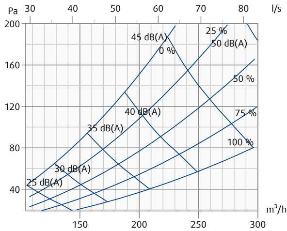
VVKR-B-S-300-8-B-SW + PB-VVK-S-300-160-S-H-D1
