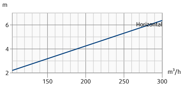
VVKR-B-S-300-8-B-SW + PB-VVK-S-300-160-S-H-D1
