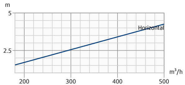
VVKR-B-S-400-16-B-SW + PB-VVK-S-400-200-S-H-D1
